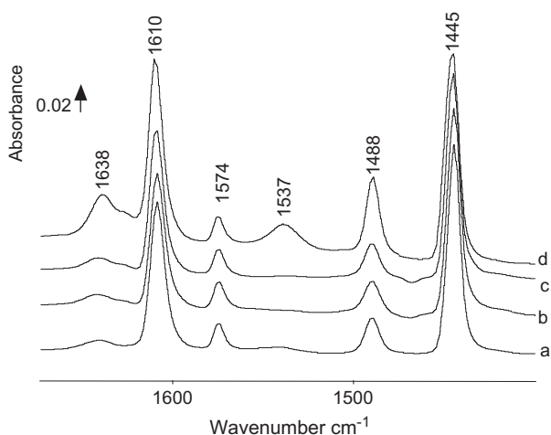
Figure 10 FTIR pyridine adsorption spectra followed of an evacuation at 373 K on: (a) (4%) V/ZrO 2 , (b) (5%) V/ZrO 2 , (c) (6%) V/ZrO 2 , (d) (7%) V/ZrO 2 .
