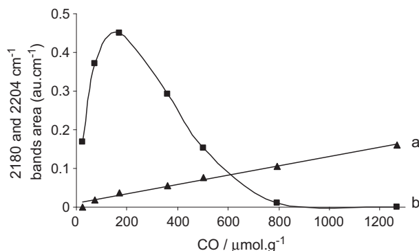
Figure 6 Evolution of the 2180 and 2204 \text{cm}^{-1} bands \text{cm}^{-1} bands area ( \text{au cm}^{-1} ) with CO content introduced in 7% \text{V}_2\text{O}_5/\text{ZrO}_2 . (a) 2180 \text{cm}^{-1} band and (b) 2204 \text{cm}^{-1} band.
