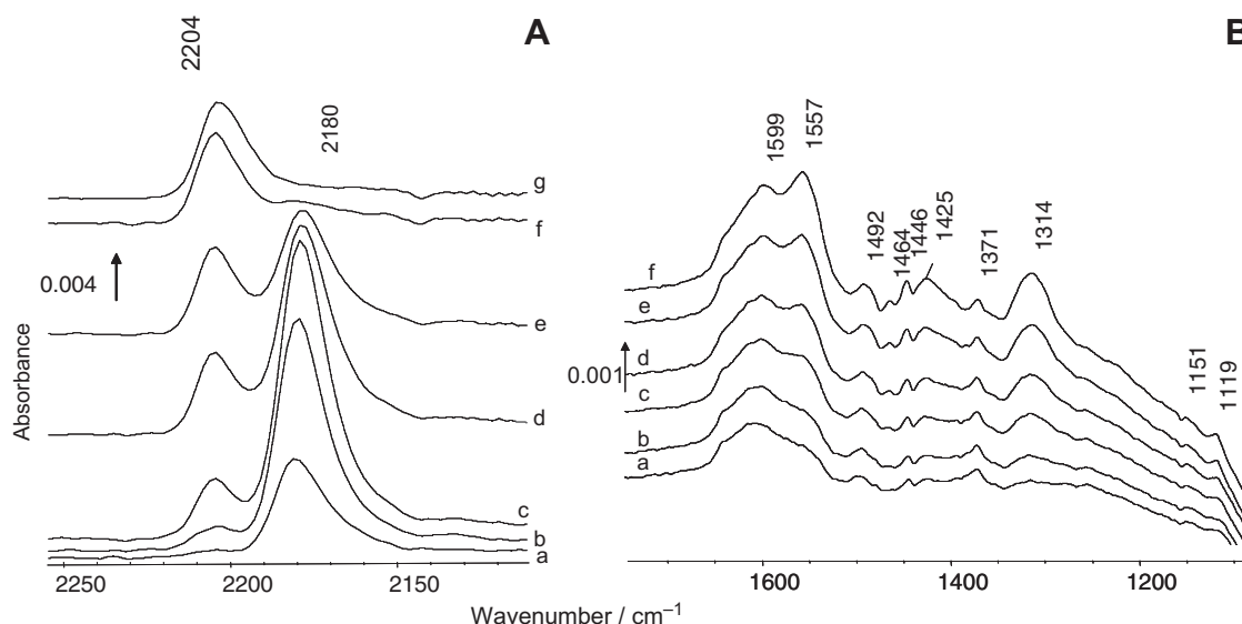
Figure 5 FT-IR spectra obtained after adsorption of successive doses of CO on (7%) \text{V}_2\text{O}_5/\text{ZrO}_2 reduced by \text{H}_2 at 723 K: (a) 24, (b) 74, (c) 168, (d) 358, (e) 503, (f) 793 and (g) 1268 \mu\text{mol/g} . (A) 2300–2100 \text{cm}^{-1} range, (B) 1700–1100 \text{cm}^{-1} range.
