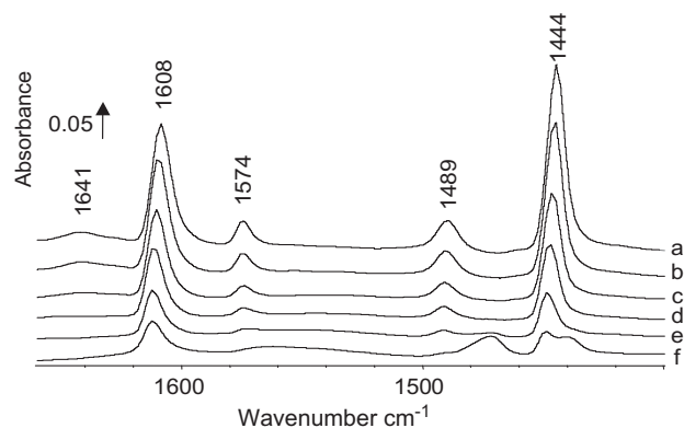
Figure 9 FTIR pyridine adsorption spectra on (5%) V/ZrO 2 followed of an evacuation at: (a) 373 K (b) 423 K, (c) 473 K, (d) 523 K, (e) 573 K and (f) 623 K.
