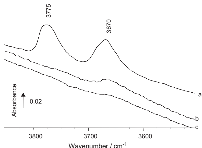
Figure 1 FT-IR spectra in the \nu(OH) range, after O_2 oxidation at 723 K of the samples: (a) ZrO_2 , (b) 5% V_2O_5/ZrO_2 and (c) 7% V_2O_5/ZrO_2 .
