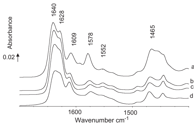
Figure 11 The adsorption of 2,6-DMP followed of an evacuation at (a) r.t, (b) 373 K, (c) 423 K and (d) 473 K on (7%) V 2 O 5 /ZrO 2 activated at 723 K.
