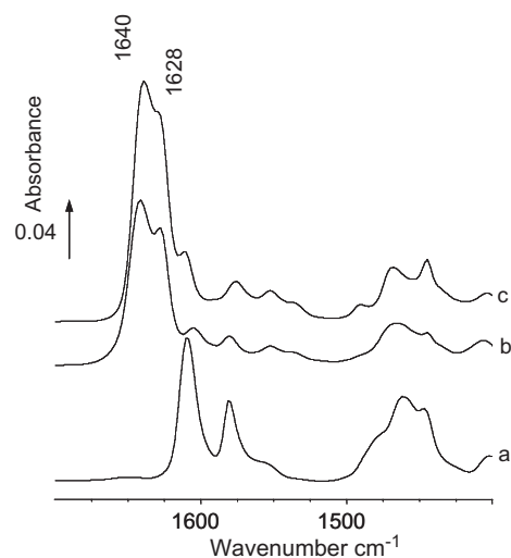
Figure 12 The adsorption of 2,6-DMP followed of an evacuation at 373 K on ZrO 2 , (7%) V 2 O 5 /ZrO 2 and (4%) V 2 O 5 /ZrO 2 activated under vacuum at 423 K: (a) ZrO 2 , (b) (4%) V 2 O 5 /ZrO 2 , (c) (7%) V 2 O 5 /ZrO 2 .
