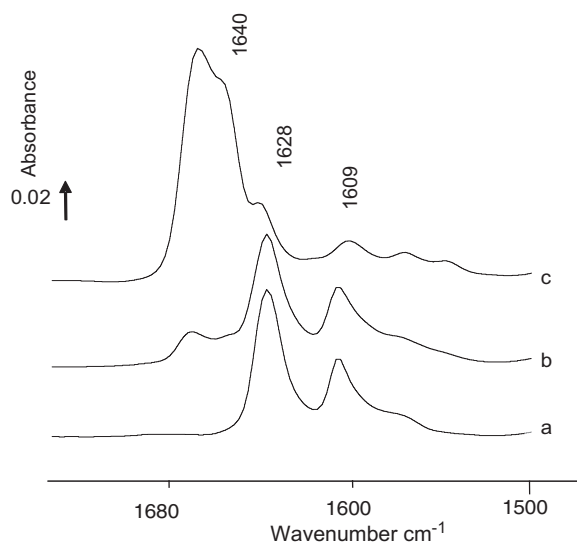
Figure 13 2,6-DMP of adsorption on ZrO 2 and (7%) V 2 O 5 /ZrO 2 followed an evacuation at 423 K: (a) ZrO 2 , (b) V 2 O 5 /ZrO 2 activated under H 2 , (c) V 2 O 5 /ZrO 2 activated under O 2 .
