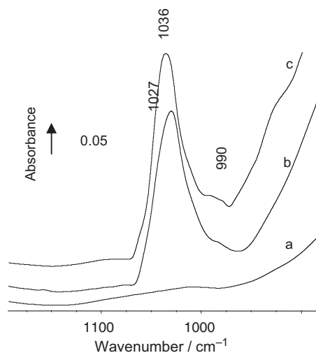
Figure 2 FT-IR spectra after activation under O_2 at 723 K of samples: (a) pure ZrO_2 , (b) 5% V_2O_5/ZrO_2 and (c) 7% V_2O_5/ZrO_2 .
