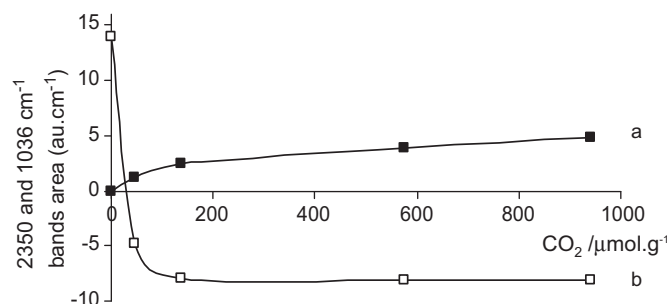
Figure 8 Evolution of the 2350 and 1036 cm -1 bands area (au cm -1 ) with CO 2 content introduced in 7% V 2 O 5 /ZrO 2 , (a) 2350 cm -1 band and (b) 1036 cm -1 band.
